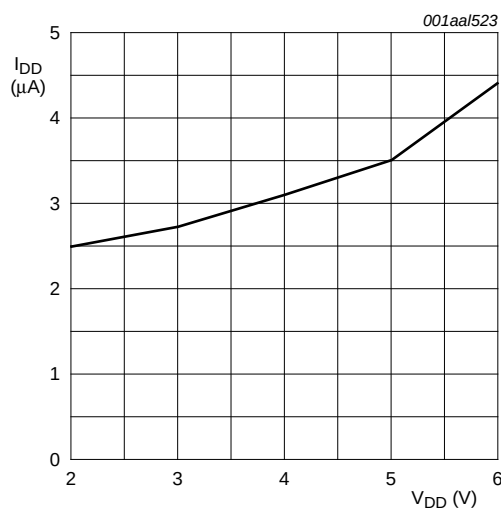
Fig 24. Typical I_{DD} with respect to V_{DD}
