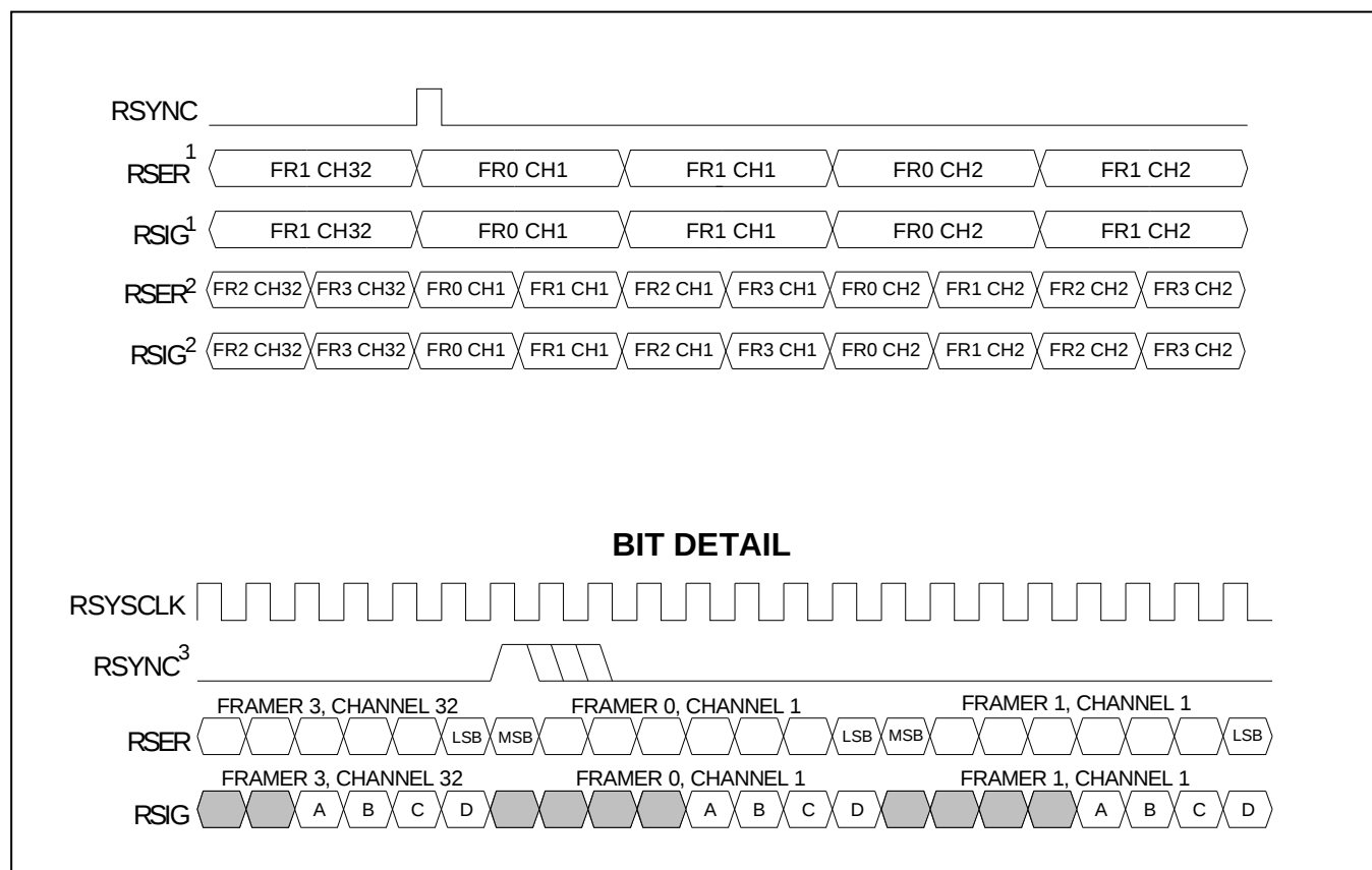
Figure 36-15. Receive IBO Channel Interleave Mode Timing
