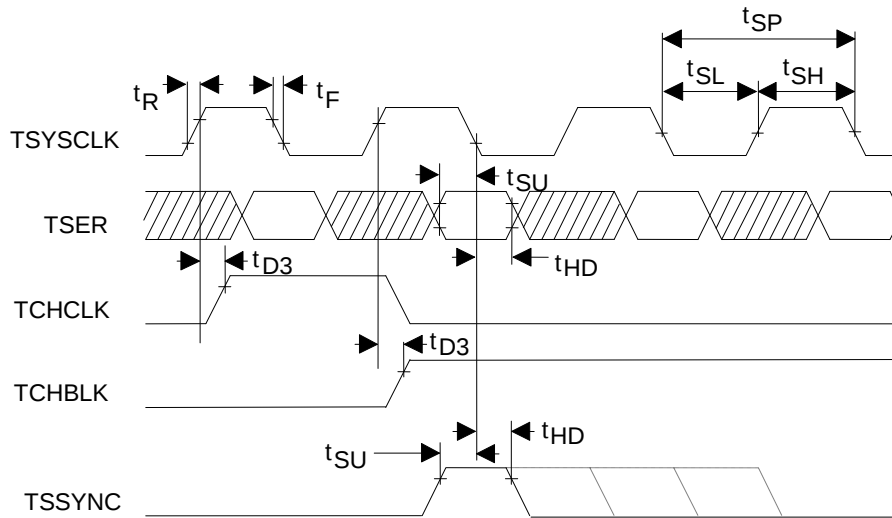
Figure 38-14. Transmit Side Timing, Elastic Store Enabled
