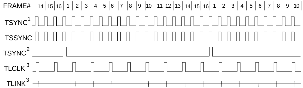
Figure 36-18. Transmit Side Timing
