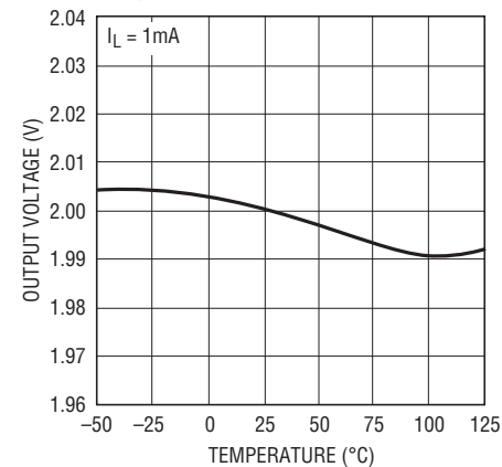
LT1761-2 Output Voltage
