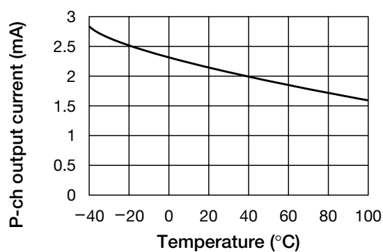
P-ch output current temperature ( V_{DS} = 0.5V )
