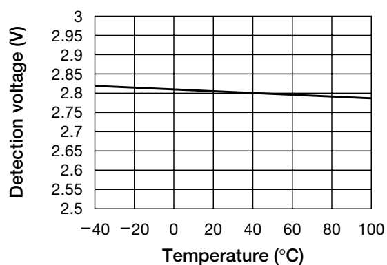
Detection voltage temperature
