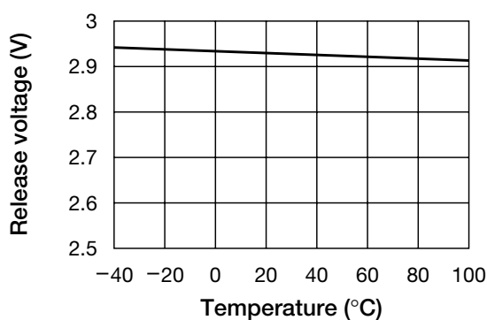
Release voltage temperature
