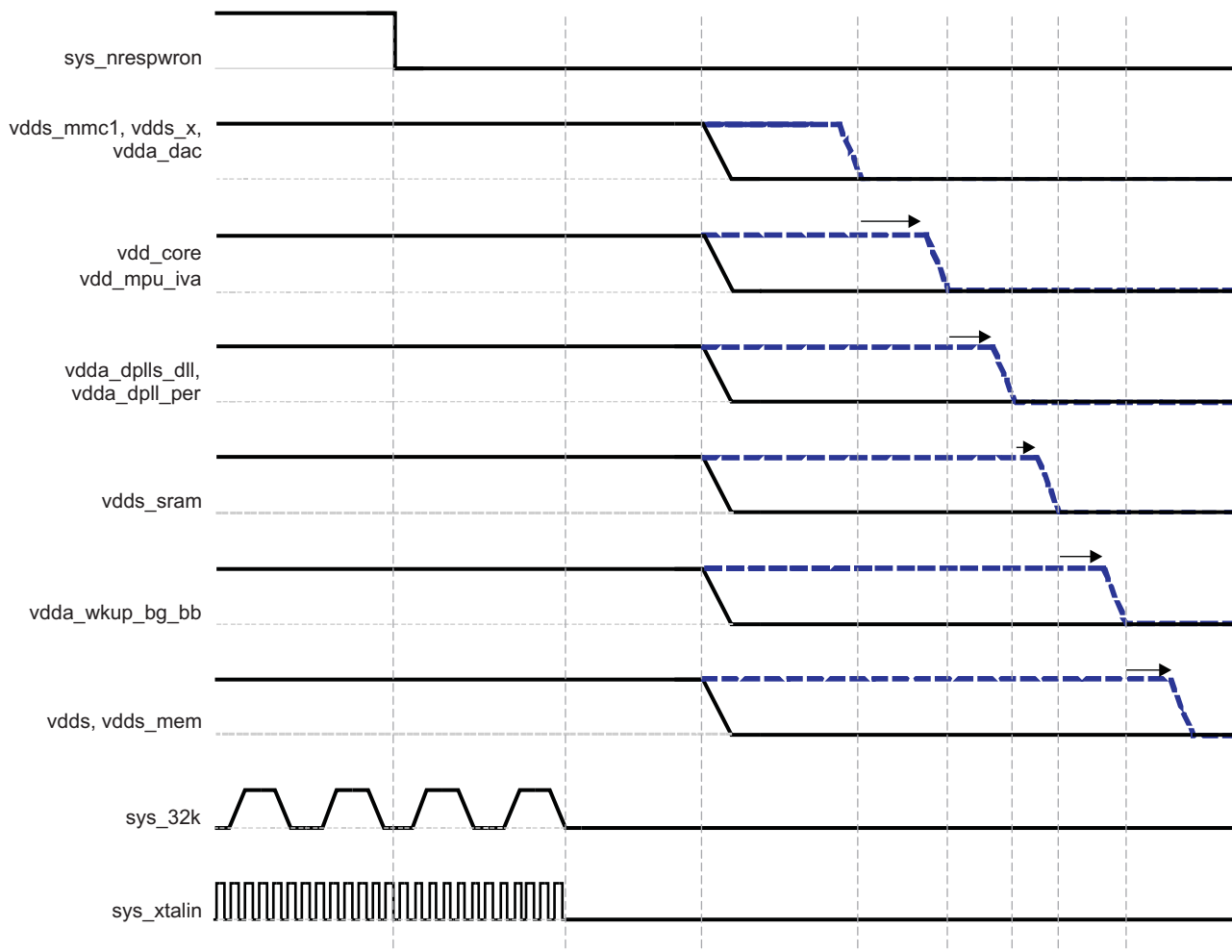
Figure 3-3. Power-Down Sequence
