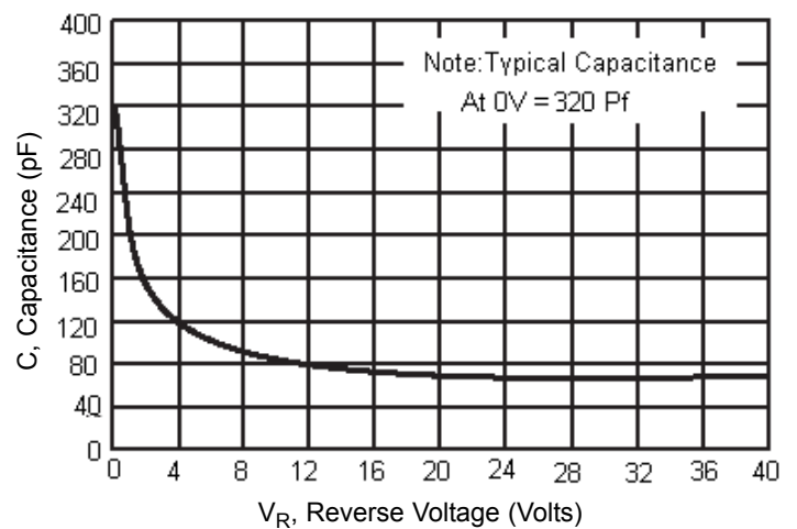
Typical Capacitance
