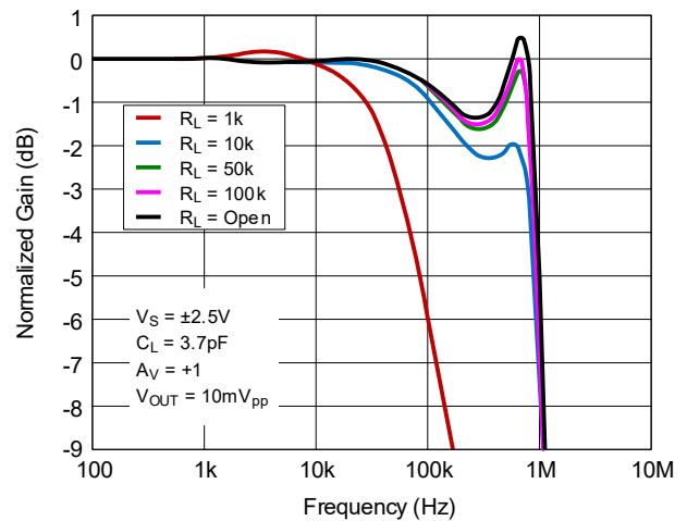
Figure 10. Gain Response vs Load Resistance, V_S = \pm 2.5V
