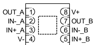
8 Ld DFN Top View
