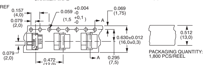
CARRIER TAPE
