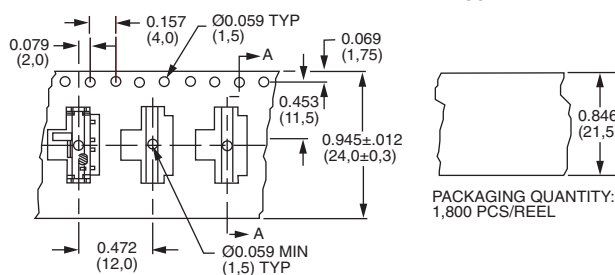
CARRIER TAPE
