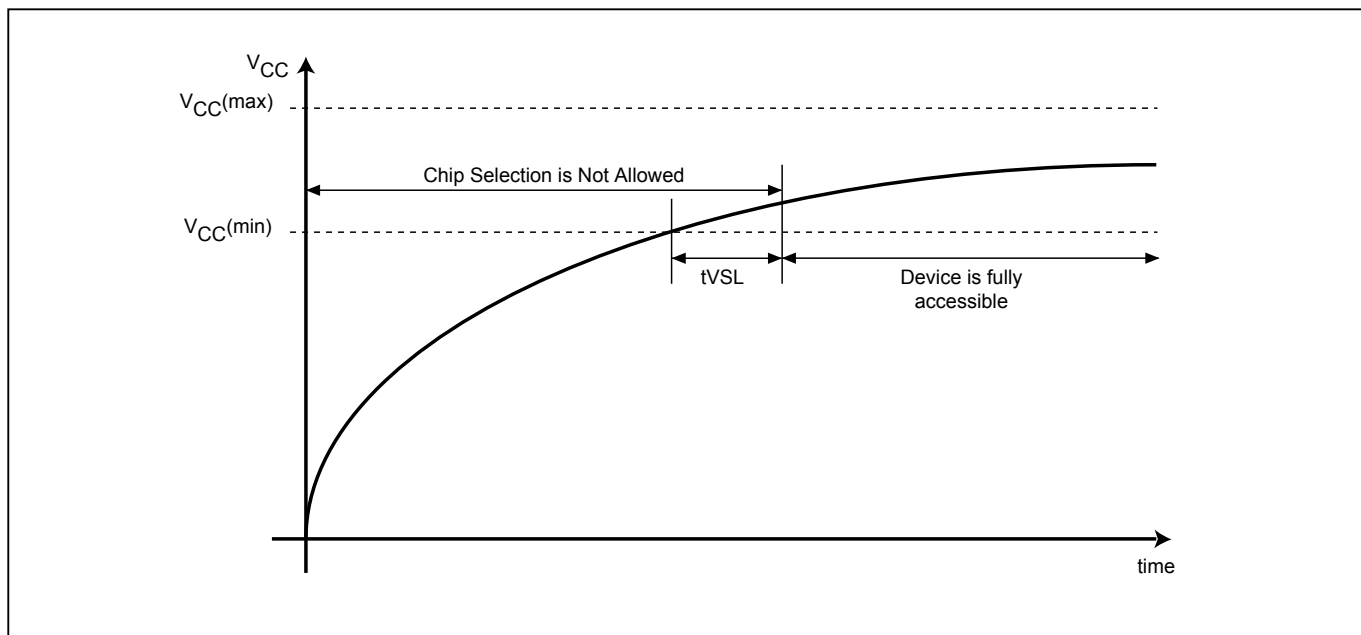
Figure 29. Power-up Timing
