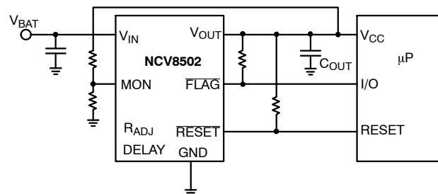
Figure 14. FLAG/Monitor Function
