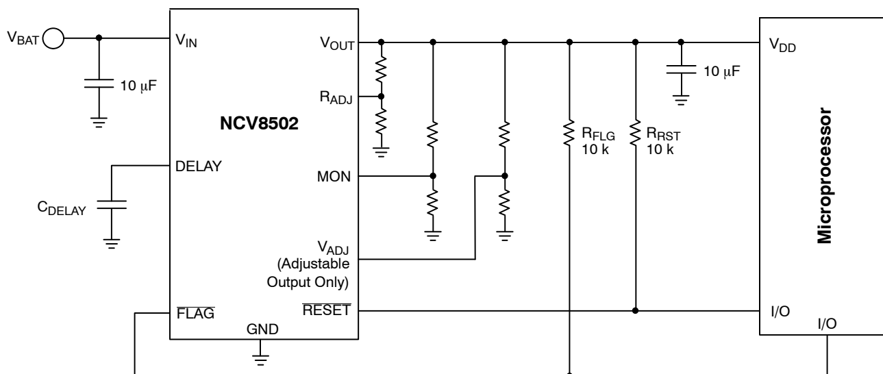
Figure 1. Application Diagram
