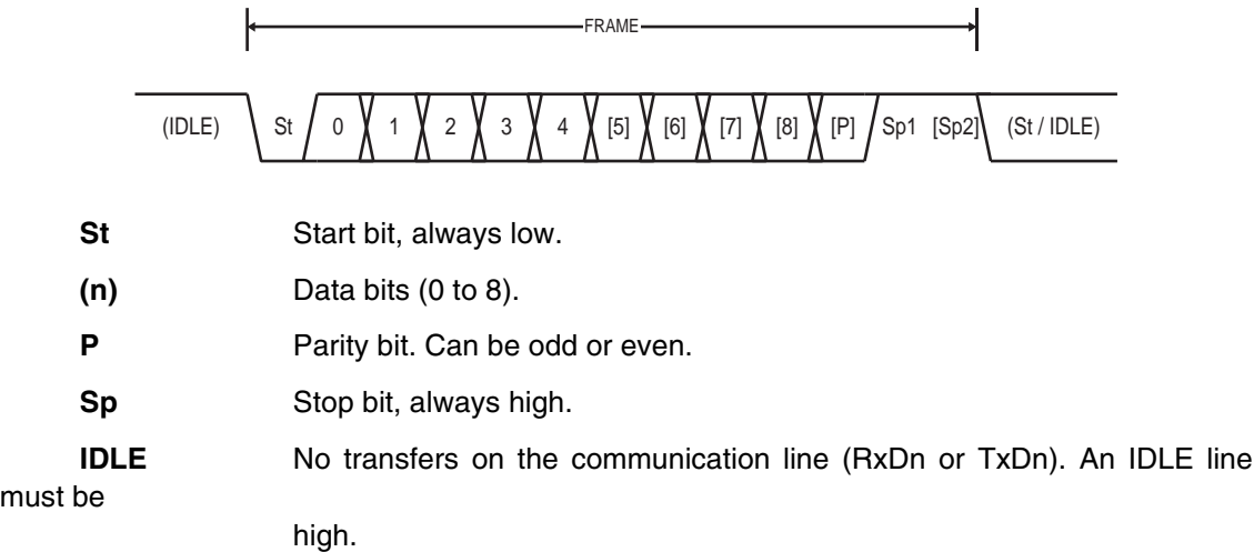
Figure 20-4. Frame Formats
