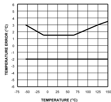
Temperature Error
