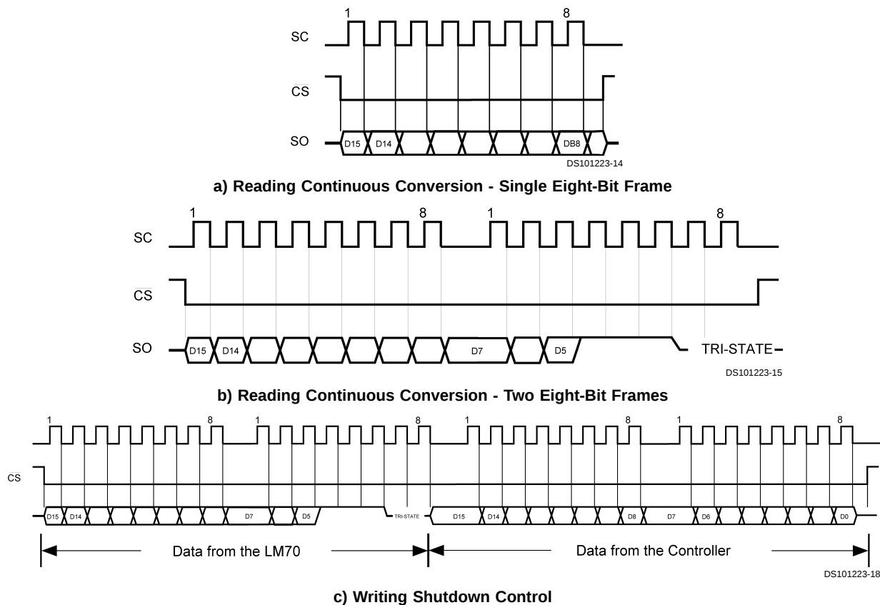
FIGURE 7. Timing Diagrams
