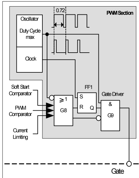
Figure 9 PWM Section
