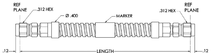
2.92 MM males on 40 GHz Workhorse® Cable
