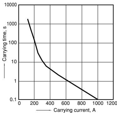
(1) Cut off current/voltage: 300A/42V DC (resistive load)
