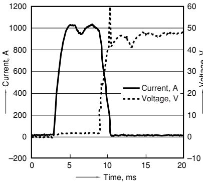
(2) Cut-off current/voltage: 1,000A/42V DC (resistive load)
