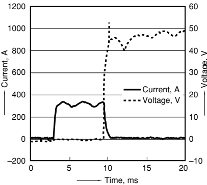
(1) Cut off current/voltage: 300A/42V DC (resistive load)
