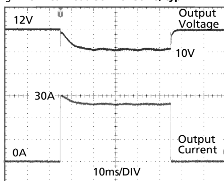
Fig. 27-3 Peak load 30A for 50ms, typ.
