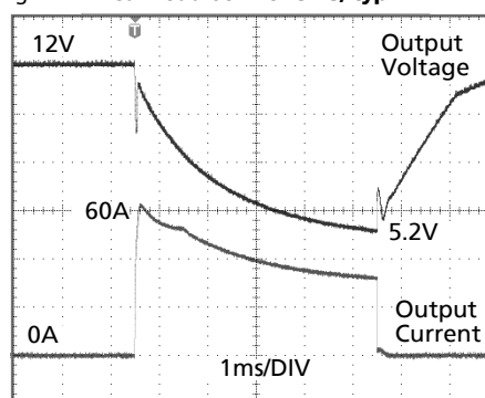
Fig. 27-4 Peak load 60A for 5ms, typ.
