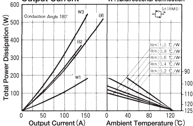
Output Current
