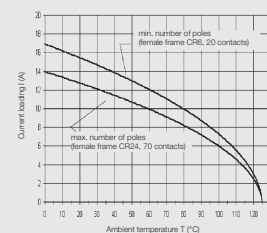
ConCept module CM-10 Conductor H07V-K 2.5 mm 2
