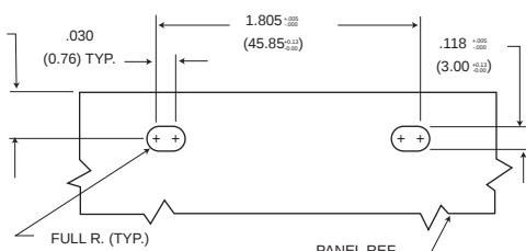
Figure 3 Edgeboard Mounting
