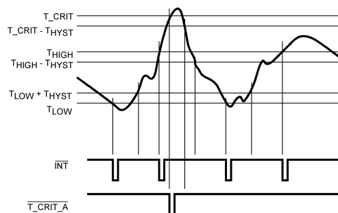
FIGURE 15. Extended One-Time Interrupt
