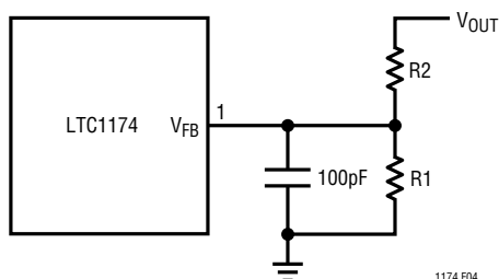
Figure 4. LTC1174 Adjustable Configuration
