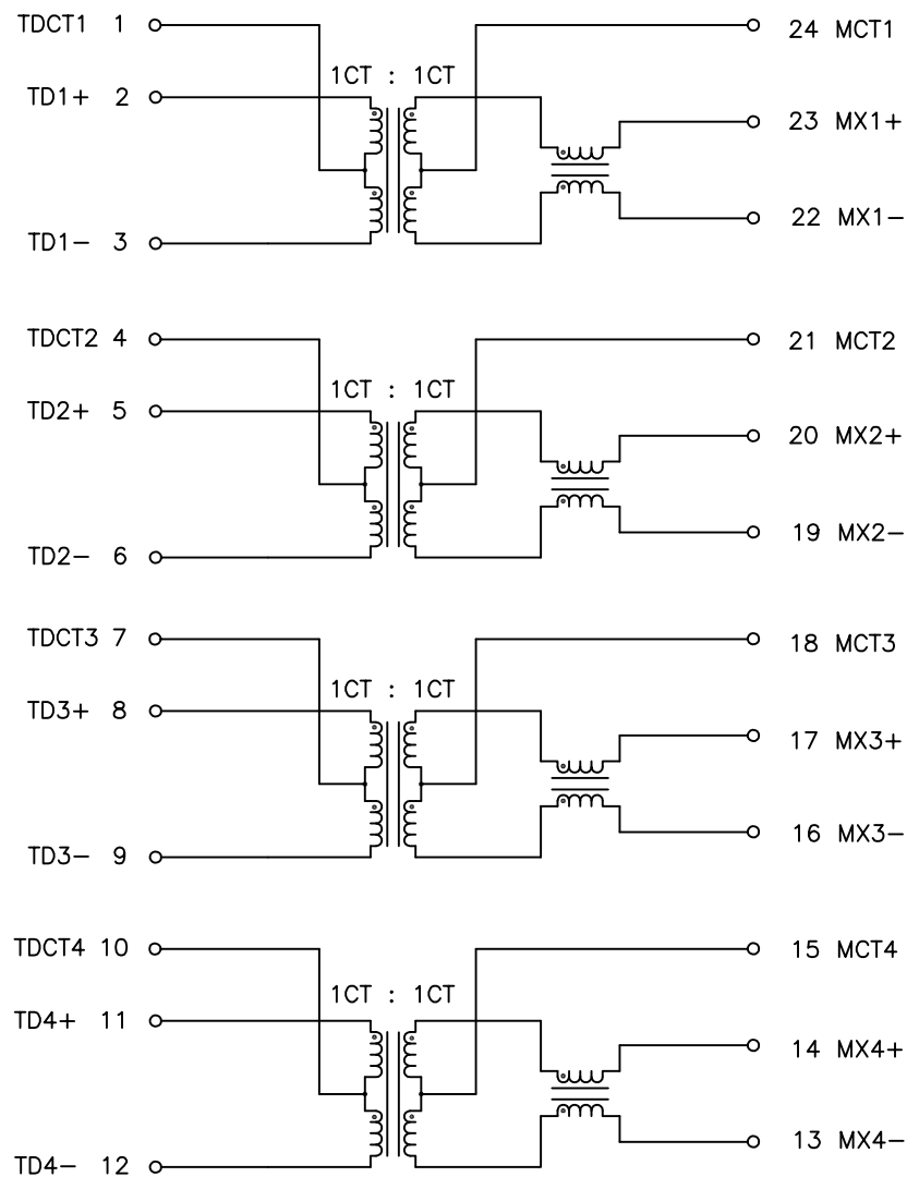
SCHEMATIC
