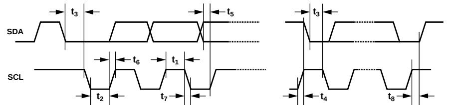
Figure 3. I²C Timing
