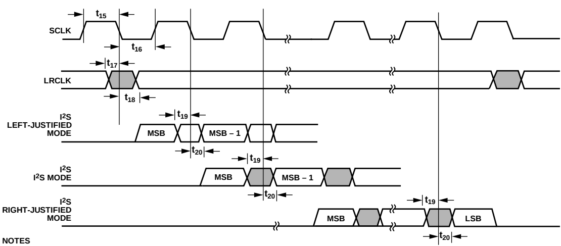
Figure 5. I²S Timing
