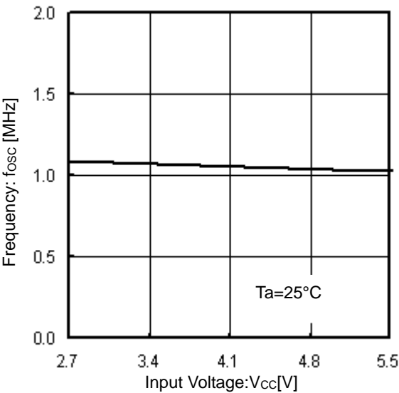
Figure 9. Frequency vs Input Voltage
