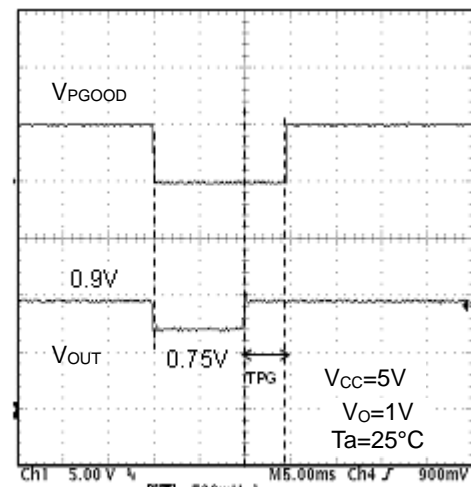
Figure 21. PGOOD Delay
