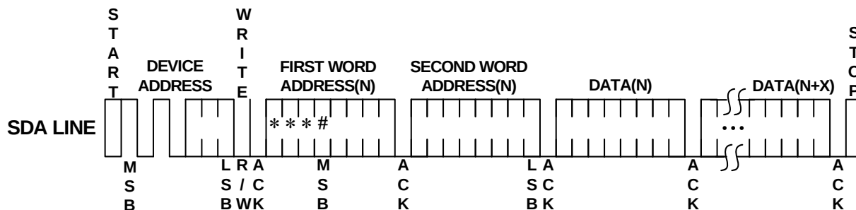
Figure 4: Page Write
