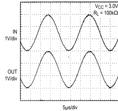
Figure 4. Rail-to-Rail Input/Output Range
