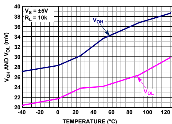
FIGURE 30. OUTPUT OVERHEAD VOLTAGE vs TEMPERATURE, V_S = \pm 5V , R_L = 10k
