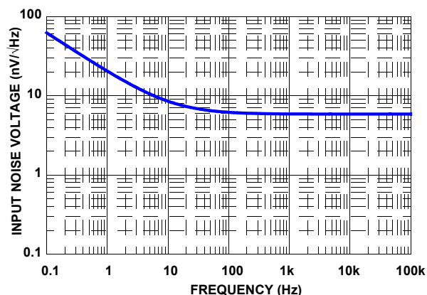
FIGURE 67. SIMULATED INPUT NOISE VOLTAGE
