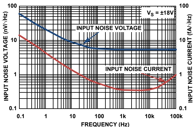
FIGURE 66. CHARACTERIZED INPUT NOISE VOLTAGE
