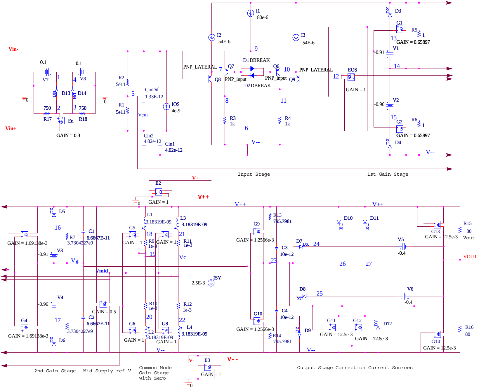
FIGURE 64. SPICE SCHEMATIC
