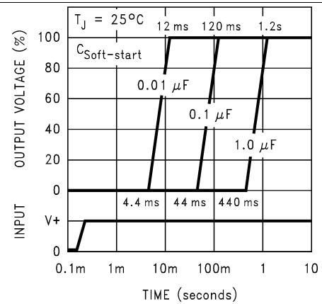
Figure 16. Soft-Start Response
