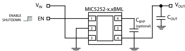
Ultra-Low-Noise Regulator Application
