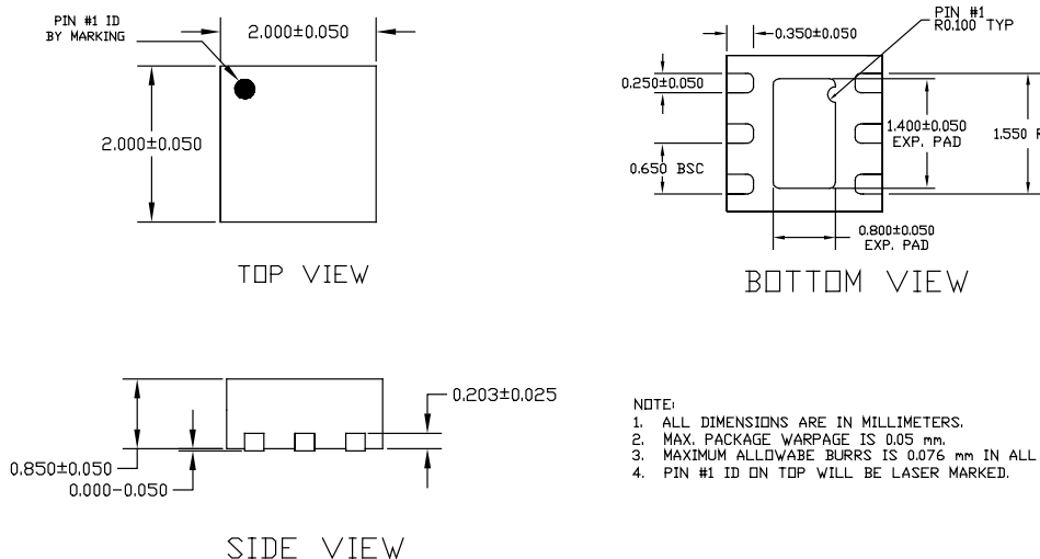
6-Pin MLF™ (ML)
