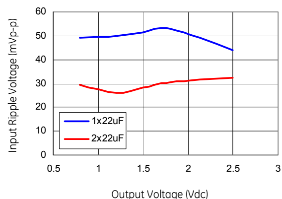
Figure 35. Input ripple voltage in mV, p-p for various output voltages with 1x22 μF or 2x22 μF ceramic capacitors at the input (3A load). Input voltage is 3.3V.
