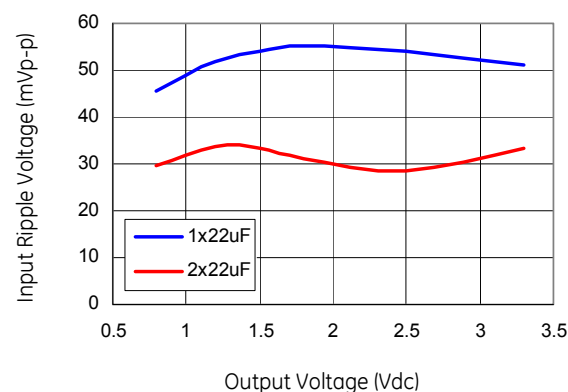
Figure 34. Input ripple voltage for various output voltages with 1x22 μF or 2x22 μF ceramic capacitors at the input (3A load). Input voltage is 5V.
