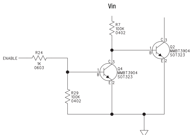
Figure 6. On/Off Control Circuit
