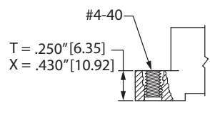
FLUSH MOUNTING WITH THREADED INSERT (T, X)
