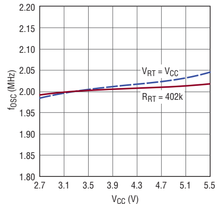
Oscillator Frequency vs V CC
