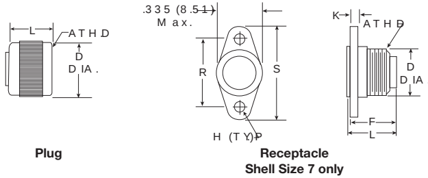
Plug
