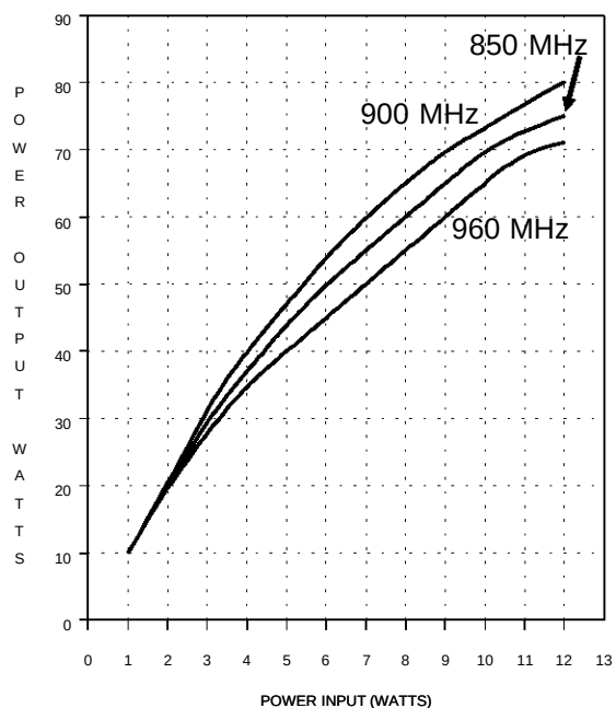
BROADBAND POWER OUTPUT vs POWER INPUT
