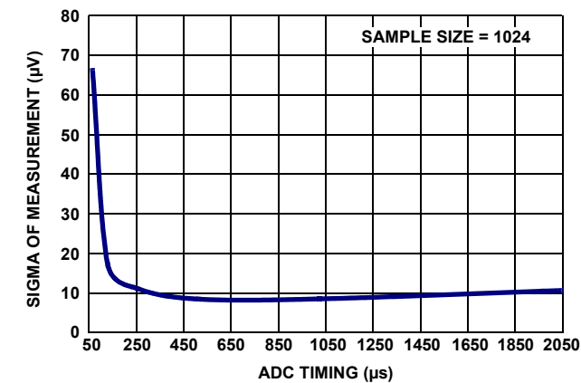
FIGURE 87. PRIMARY SHUNT STABILITY: STDEV vs ACQUISITION TIME
