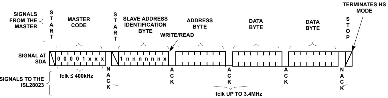
FIGURE 109. BYTE TRANSACTION SEQUENCE FOR INITIATING DATA RATES ABOVE 400kbs
