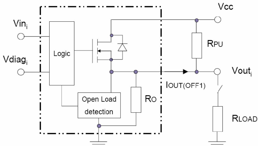
Figure 8. Open-load detection
