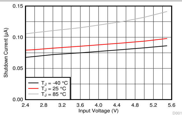
Figure 7-4. Shutdown Current
