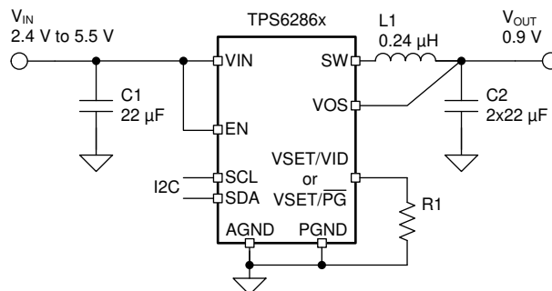
Figure 9-21. Smaller Application
