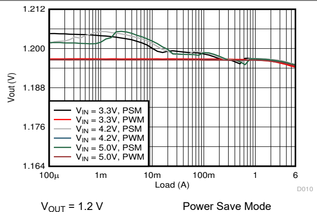
Figure 9-7. Load Regulation
