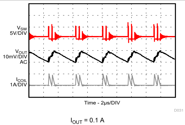
Figure 9-13. PSM Operation
