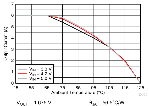
Figure 9-11. Thermal Derating
