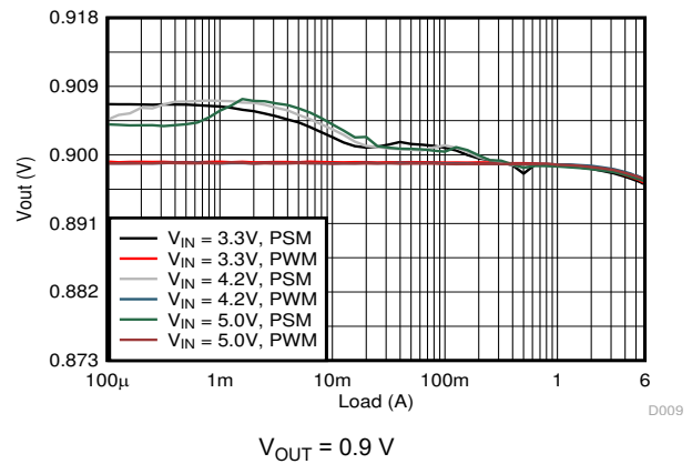
Figure 9-5. Load Regulation
