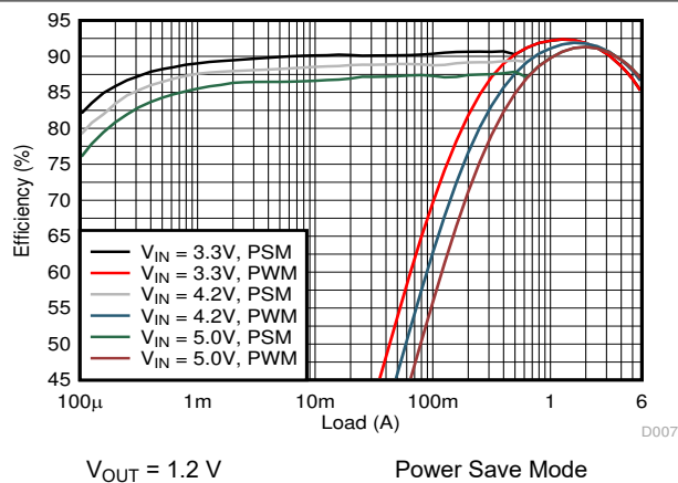
Figure 9-6. Efficiency
