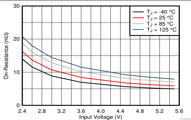
Figure 7-2. Low-Side FET On-Resistance
