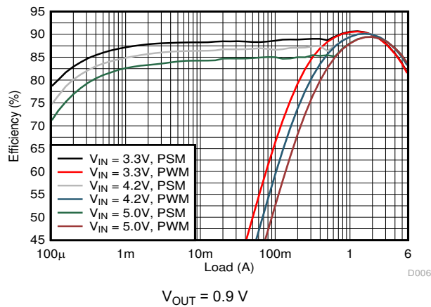
Figure 9-4. Efficiency
