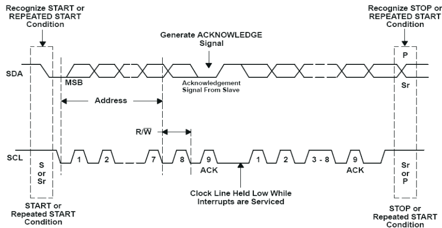
Figure 8-5. Bus Protocol
