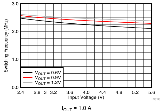
Figure 9-9. Switching Frequency
