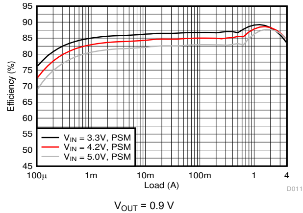
Figure 9-22. Efficiency
