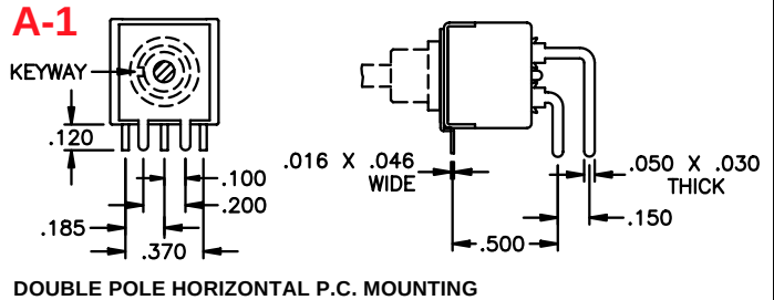
FRONT VIEW DOUBLE POLE
