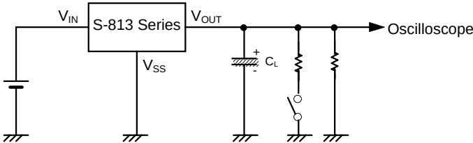
Figure 13 Measuring circuit
