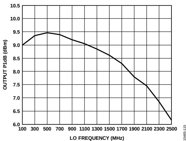
Figure 13. Output P1dB Compression Point vs. LO Frequency at Nominal Conditions
