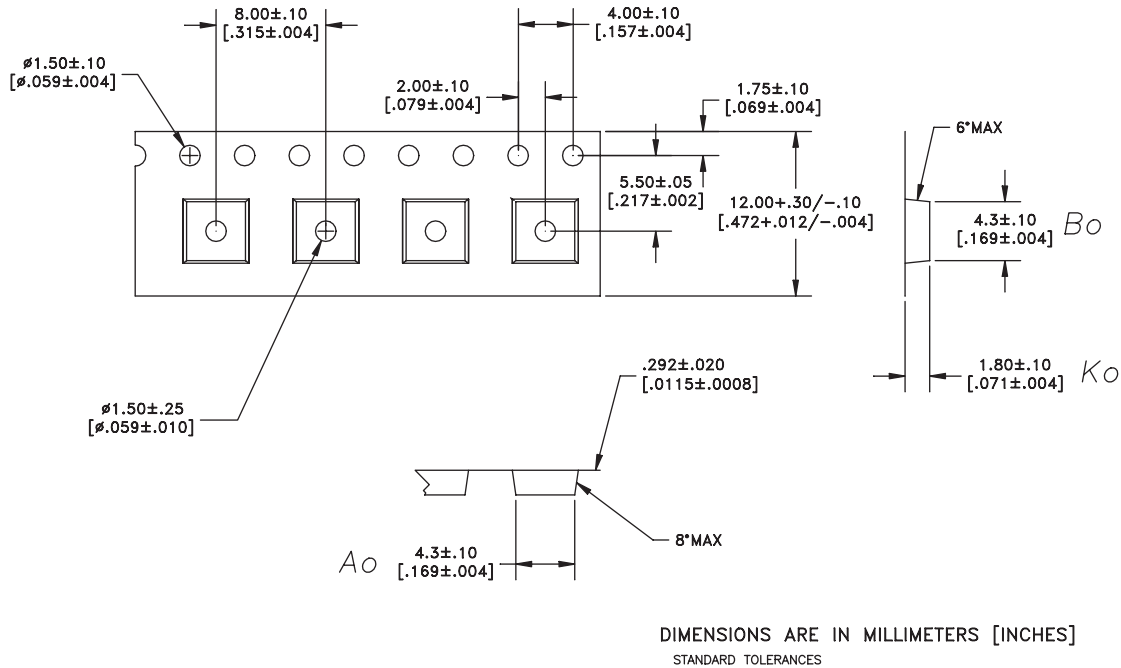
Figure 6: Tape & Reel Packaging
