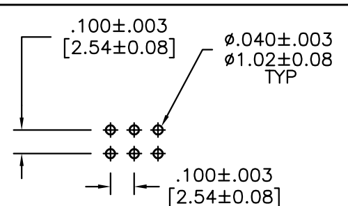
RECOMMENDED BOARD LAYOUT
