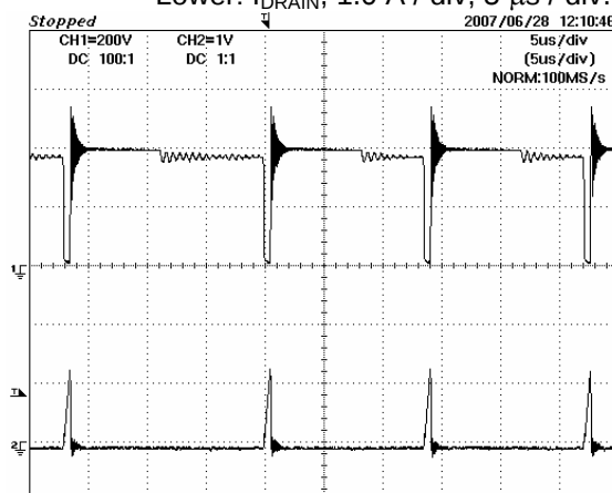
Figure 17 – 230 VAC, V_{out} = 2.3 V, I_o = 3 A Upper: V_{DRAIN} , 100 V Lower: I_{DRAIN} , 1.0 A / div, 5 \mu s / div.
