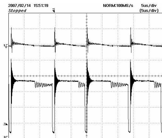
Figure 32 – 230 VAC Input, V_{out}=12 V, I_o=3 A Upper Trace: V_{out} Ripple, 500 mV / div. Lower Trace: V_{Drain} , 100 V /div. (5 \mu s / div)
