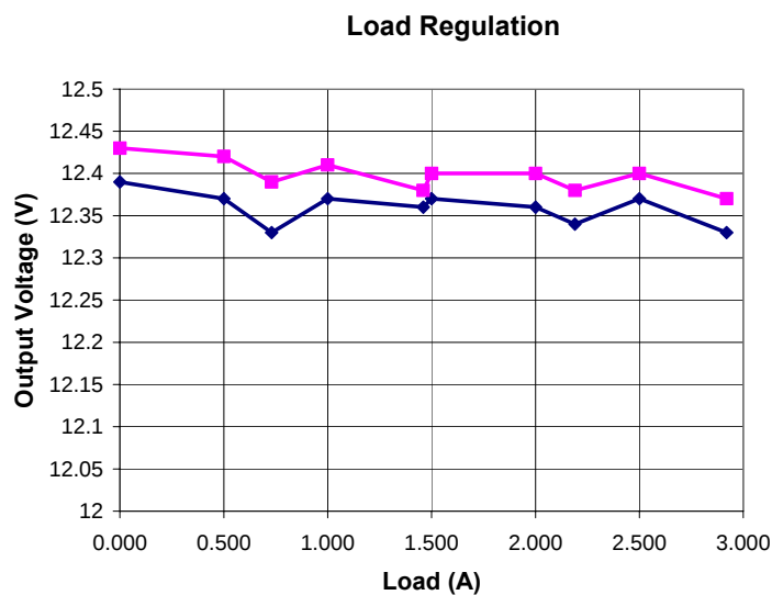
Figure 9 – Load Regulation, Room Temperature.
