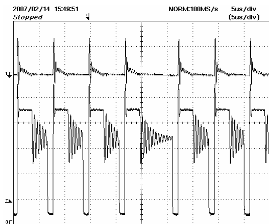
Figure 31 – 230 VAC Input, V_{out}=12 V, I_o=3 A Upper Trace: V_{out} Ripple, 500 mV / div. Lower Trace: V_{Drain} , 100 V /div. (5 \mu s / div)
