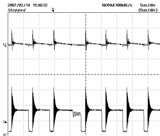
Figure 30 – 90 VAC Input, V_{out}=2.3 V, I_o=3 A Upper Trace: V_{out} Ripple, 500 mV / div. Lower Trace: V_{Drain} , 100 V /div. (5 \mu s / div)
