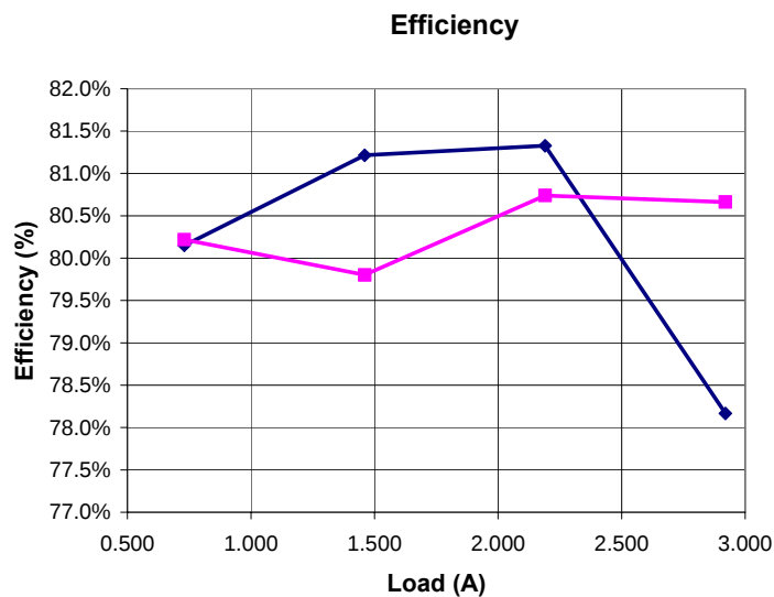
Figure 6 – Efficiency vs. Load, Room Temperature, 60 Hz.
