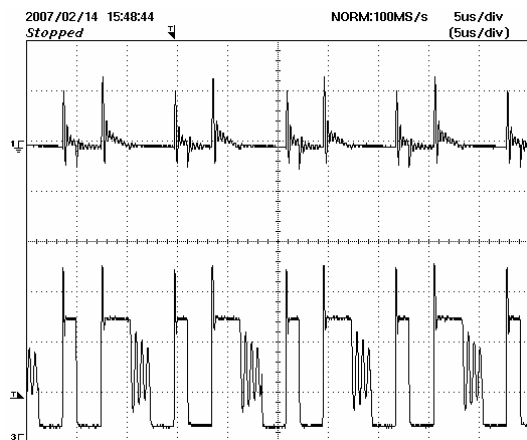
Figure 29 – 90 VAC Input, V_{out}=12 V, I_o=3 A Upper Trace: V_{out} Ripple, 500 mV / div. Lower Trace: V_{Drain} , 100 V /div. (5 \mu s / div)
