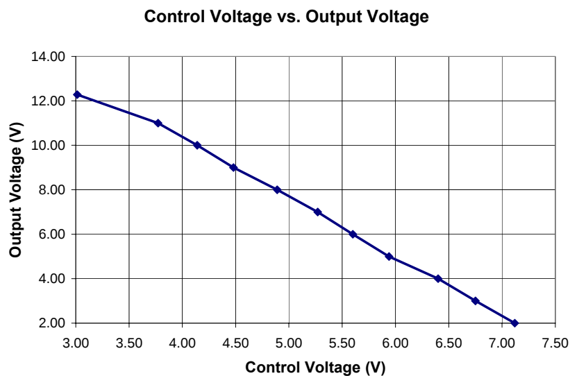
Figure 12 – Output Voltage vs. External Control Voltage.
