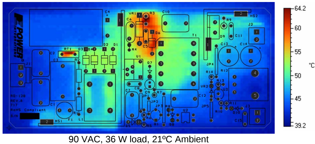
Figure 13 – Infrared Thermograph of Open Frame Operation at Room Temperature.
