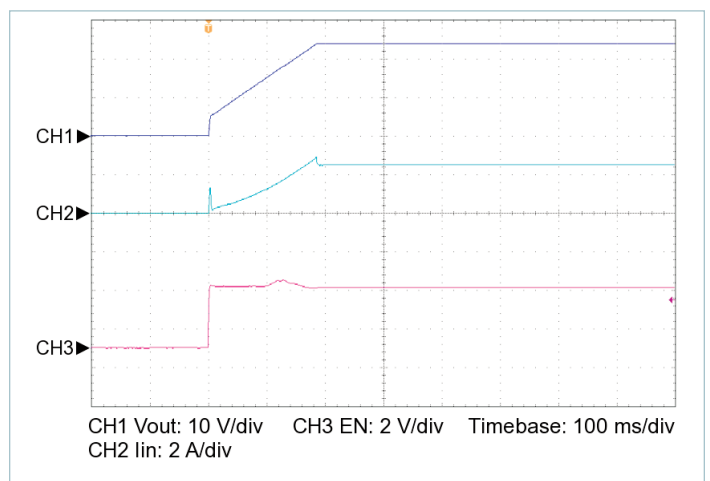
Figure 14 — Startup from EN, V_{IN} = 100\text{ V} , C_{OUT\_EXT} = 20000\text{ }\mu\text{F} , R_{LOAD} = 2.400\text{ }\Omega
