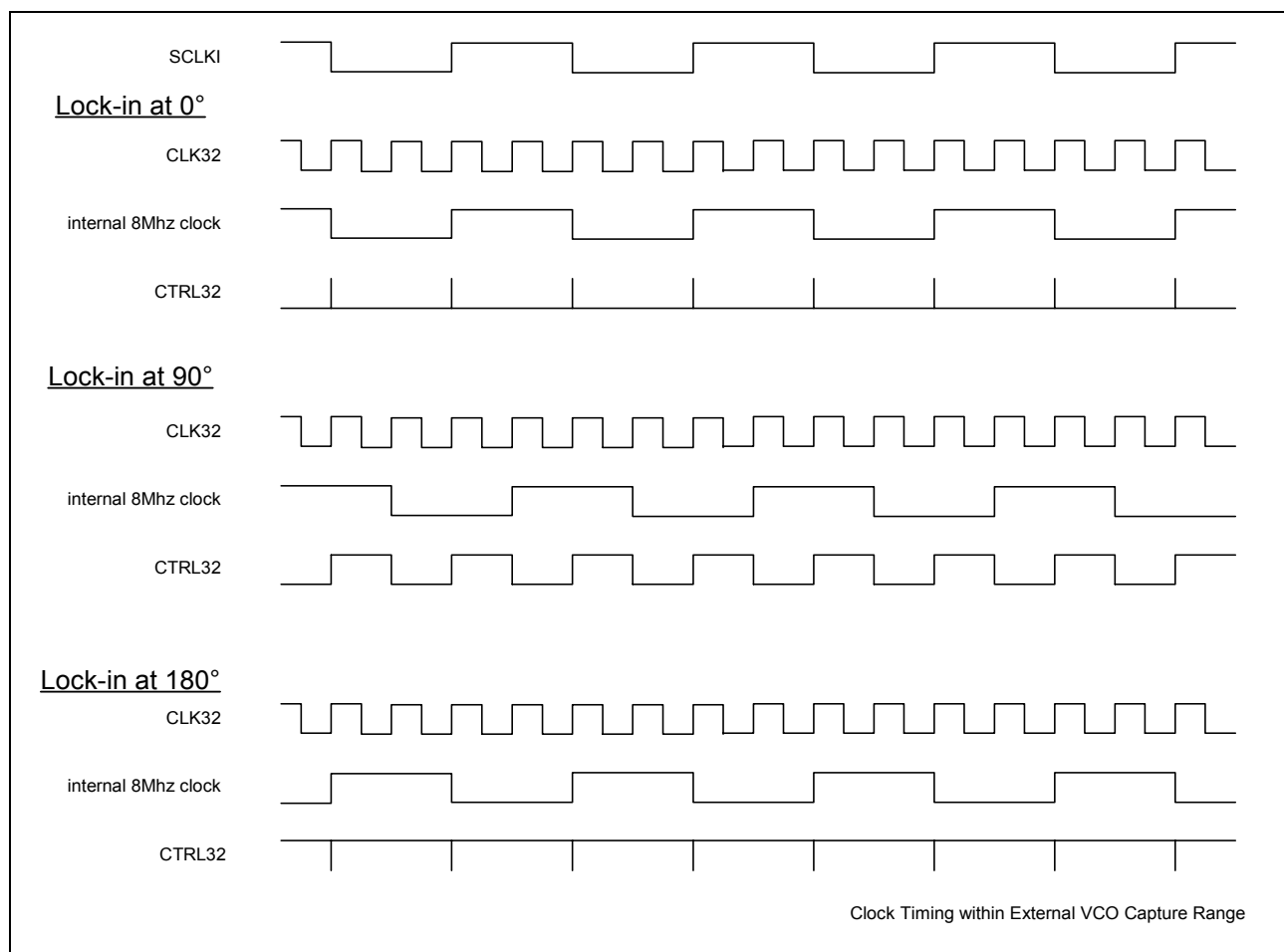
Figure 35 Clock Timing within External VCO Capture Range
