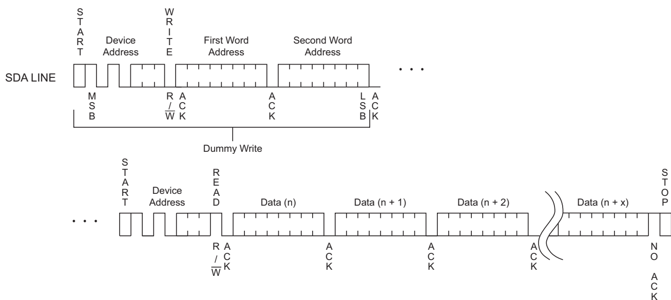
Figure 9-5. Sequential Read
