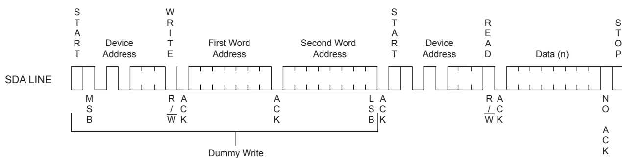
Figure 9-4. Random Read
