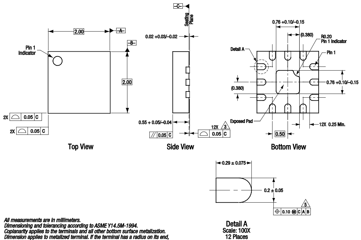
Figure 10. SKY13472-460LF 12-Pin QFN Package Dimensions
