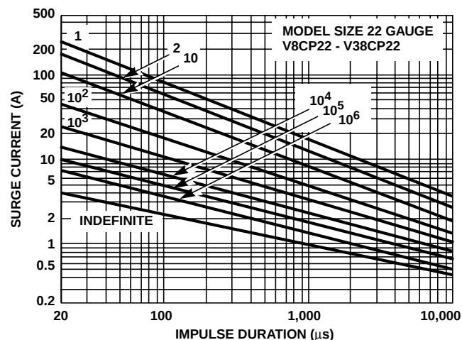
FIGURE 15. SURGE CURRENT RATING CURVES FOR V8CP22 - V38CP22
