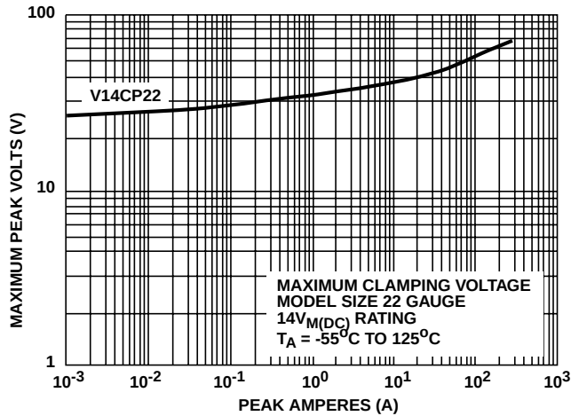
FIGURE 9. CLAMPING VOLTAGE FOR V14CP22
