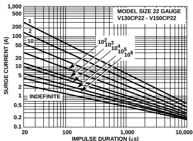
FIGURE 16. SURGE CURRENT RATING CURVES FOR V130CP22 - V150CP22
