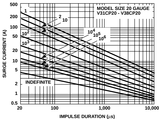
FIGURE 13. SURGE CURRENT RATING CURVES FOR V31CP20 - V38CP20
