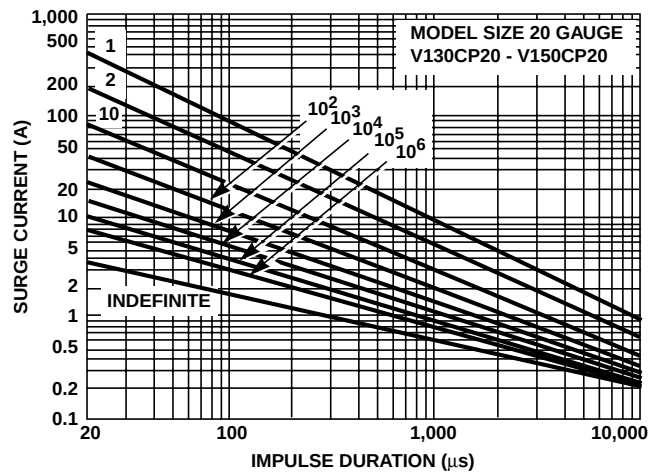
FIGURE 14. SURGE CURRENT RATING CURVES FOR V130CP20 - V150CP20
