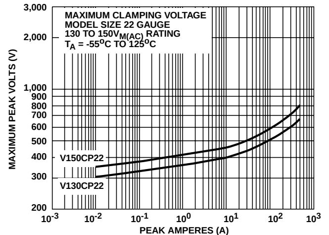
FIGURE 8. CLAMPING VOLTAGE FOR V130CP22 - V150CP22
