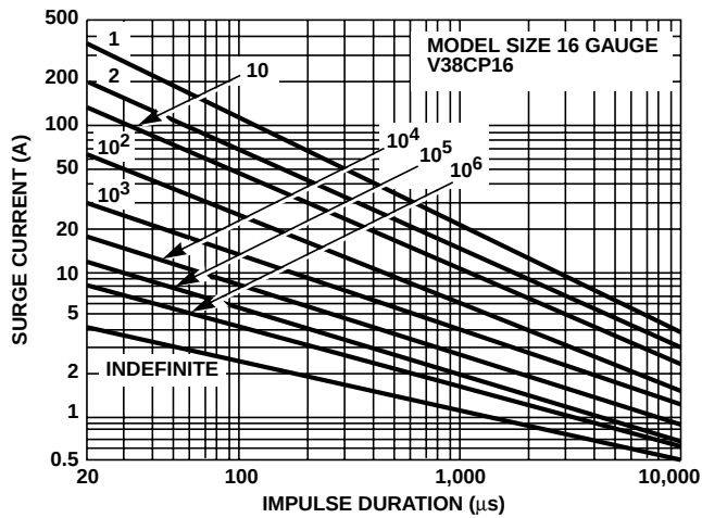
FIGURE 11. SURGE CURRENT RATING CURVES FOR V38CP16
