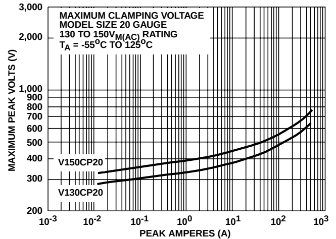
FIGURE 6. CLAMPING VOLTAGE FOR V130CP20 - V150CP20
