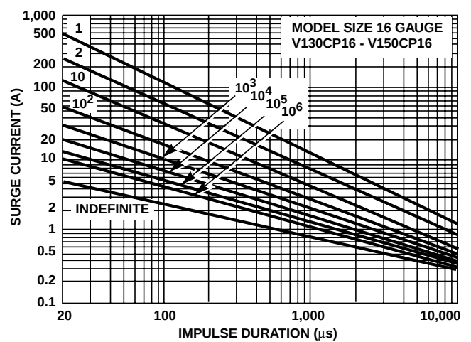
FIGURE 12. SURGE CURRENT RATING CURVES FOR V130CP16 - V150CP16
