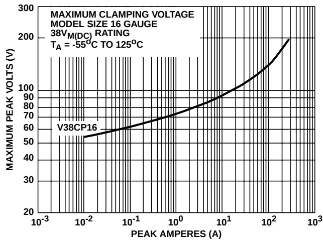
FIGURE 3. CLAMPING VOLTAGE FOR V38CP16
