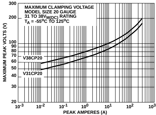
FIGURE 5. CLAMPING VOLTAGE FOR V31CP20 - C38CP20
