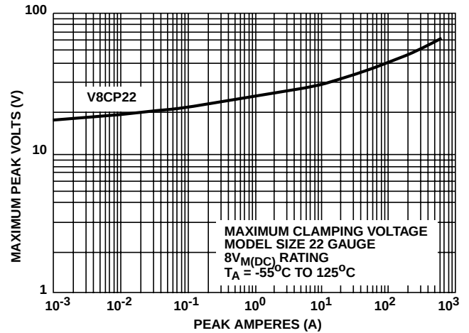
FIGURE 10. CLAMPING VOLTAGE FOR V8CP22
