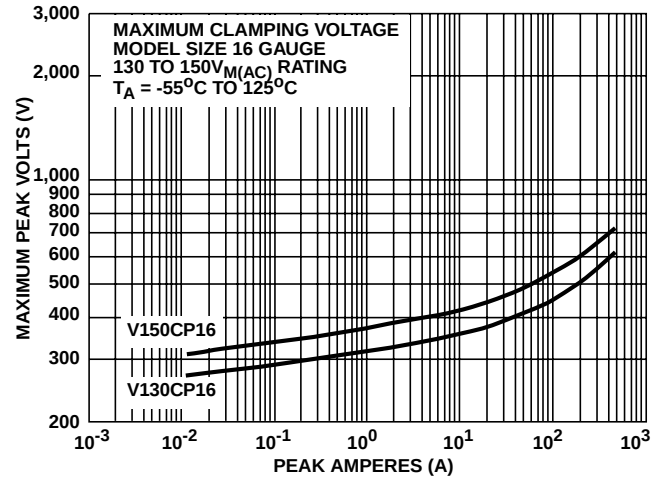
FIGURE 4. CLAMPING VOLTAGE FOR V130CP16 - V150CP16
