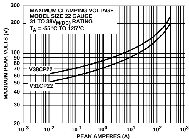
FIGURE 7. CLAMPING VOLTAGE FOR V31CP22 - V38CP22
