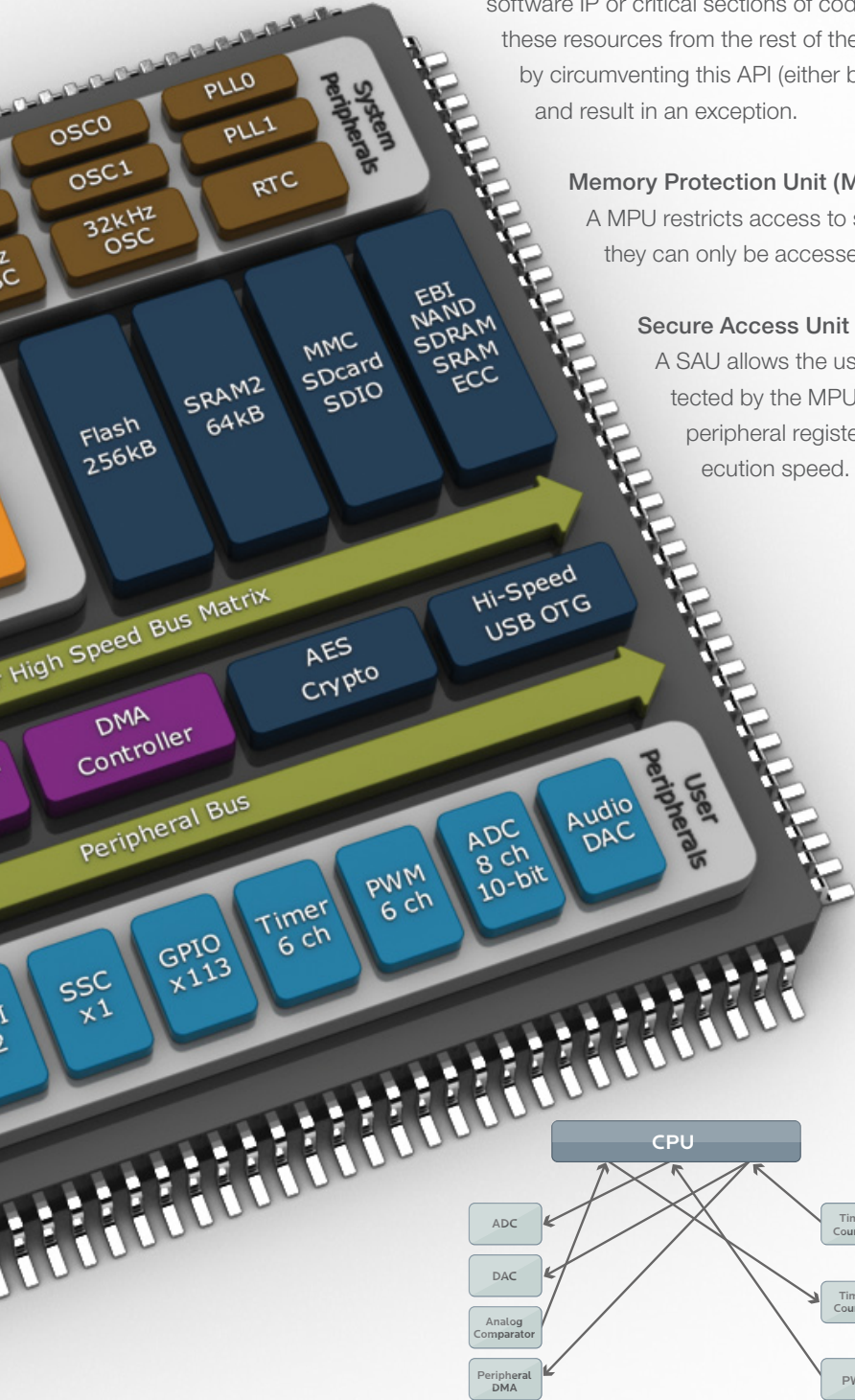
Without Peripheral Event System all Peripheral Requests need to be handled by the CPU.
